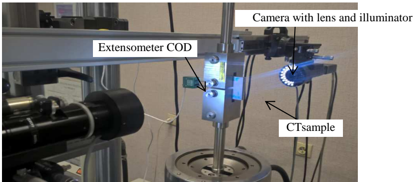
Fig. 3. Measurement stand
