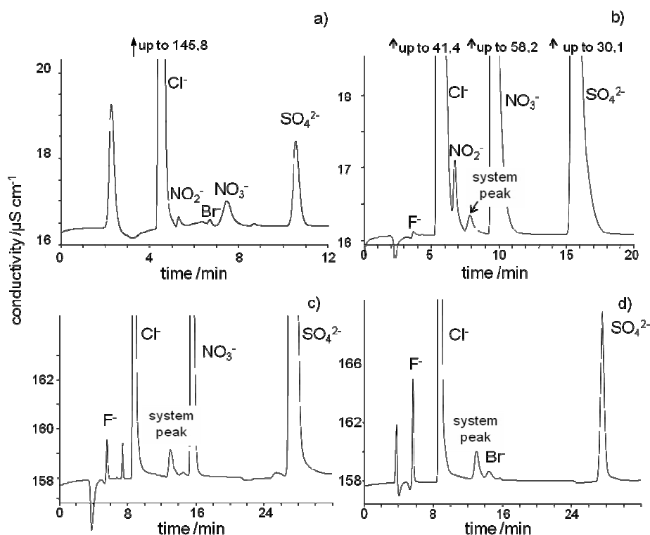
Fig. 3. The ion chromatograms of examined water samples: (a) medicinal, (b) well, (c) tap, and (d) Oligocene (Metrosep A Supp 5 Metrohm column, 3.2 mmol L -1 Na 2 CO 3 + 1.0 mmol L -1 NaHCO 3 (0.7 mL min -1 ) eluent and different column length: a, b 150 mm and c, d 250 mm)
