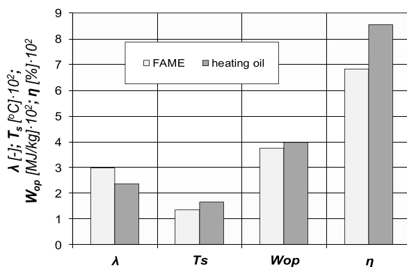
Fig. 13. The comparison between power efficiency for FAME and heating oil
