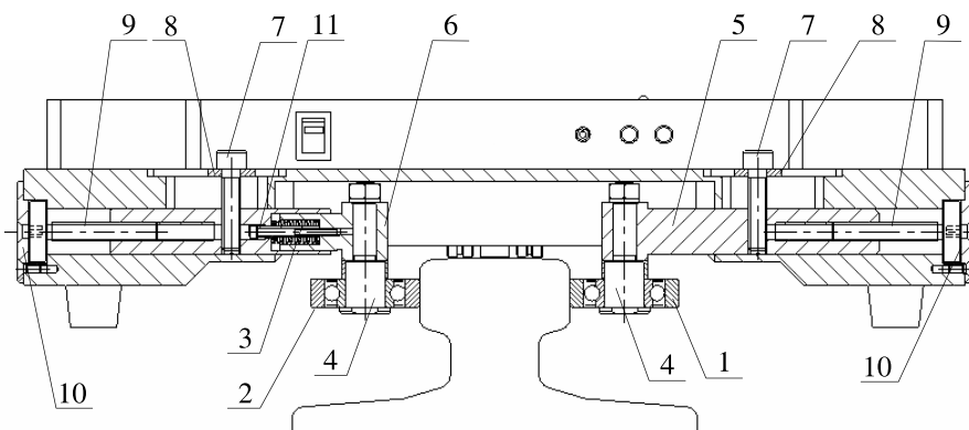
Fig. 8. A cross-section of the platform: 1 - guiding roller, 2 - pressure roller, 3 - spring, 4 - roller axis, 5 - idler guiding roller bracket, 6 – pressure roller bracket, 7 - blocking screw, 8 - board with a scale, 9 - adjusting screw, 10 - cover, and 11 - limiting screw.
