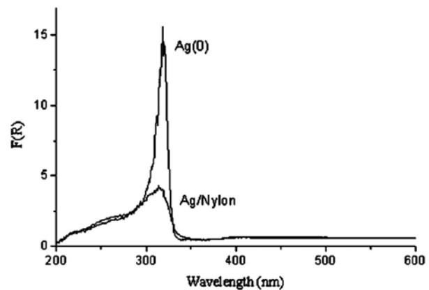
Fig. 3. Diffuse reflection spectra of a silver–nylon composite
